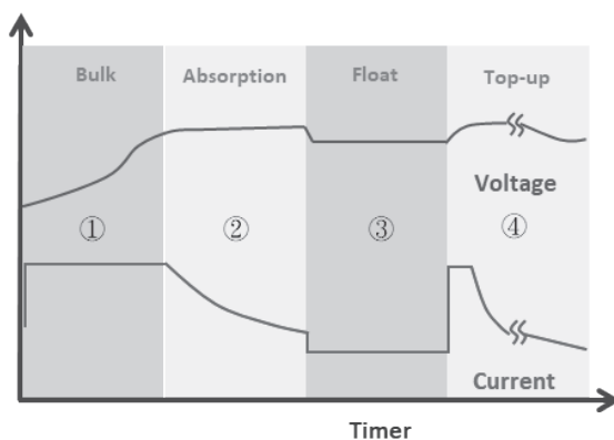
Charge Curve
