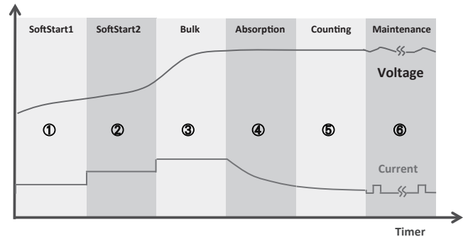
Charging Curve
