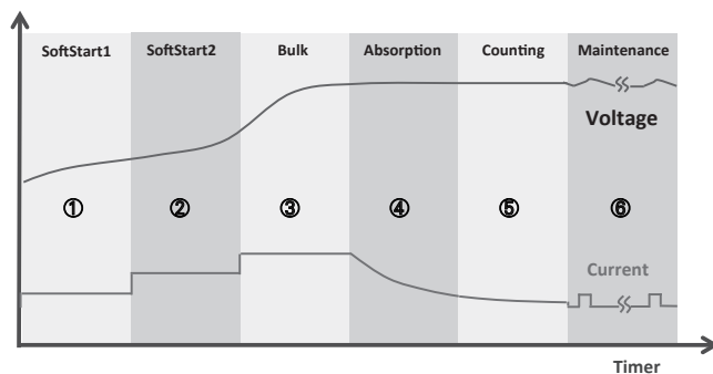
Charge Curve
