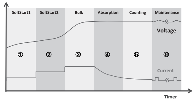
Charge Curve
